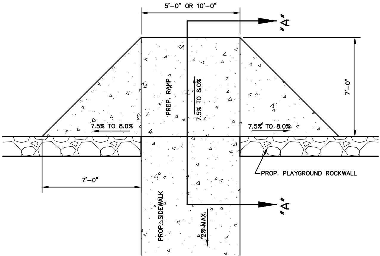
PLAYGROUND RAMP NTS
